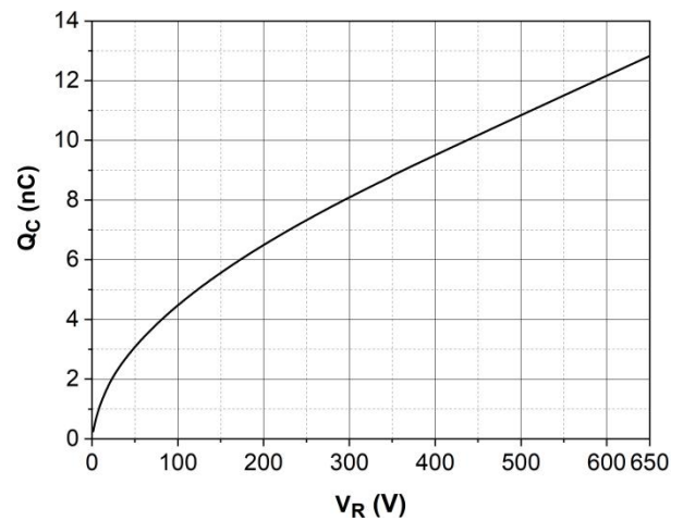
Figure 4. Recovery Charge vs. Reverse Voltage
